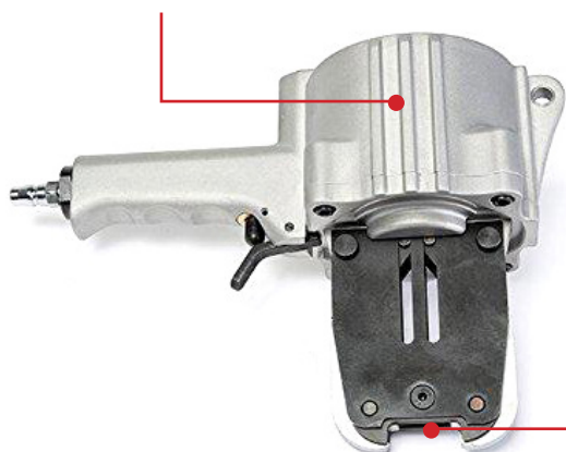
CILINDRO ARIA AIR CYLINDER
